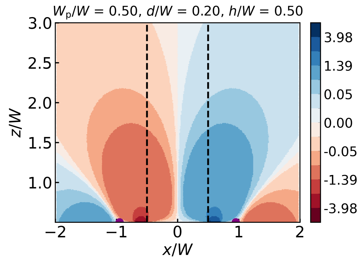
dV/dx as a function of (x,z) :
