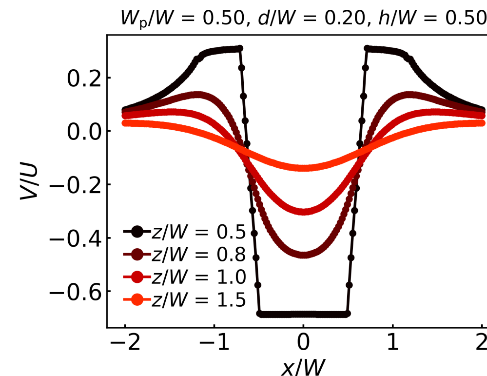
Cuts for different z :
