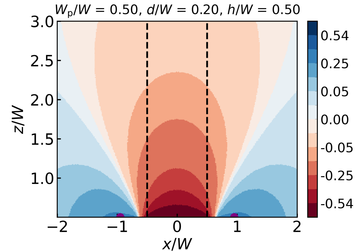
Potential as a function of (x,z) :
