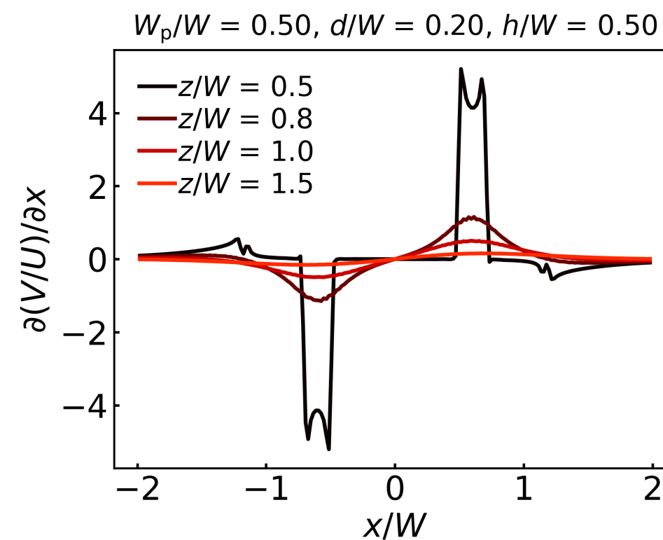
Cuts for different z :
